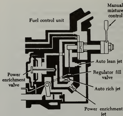
FIGURE 3-19. Fuel control unit.
